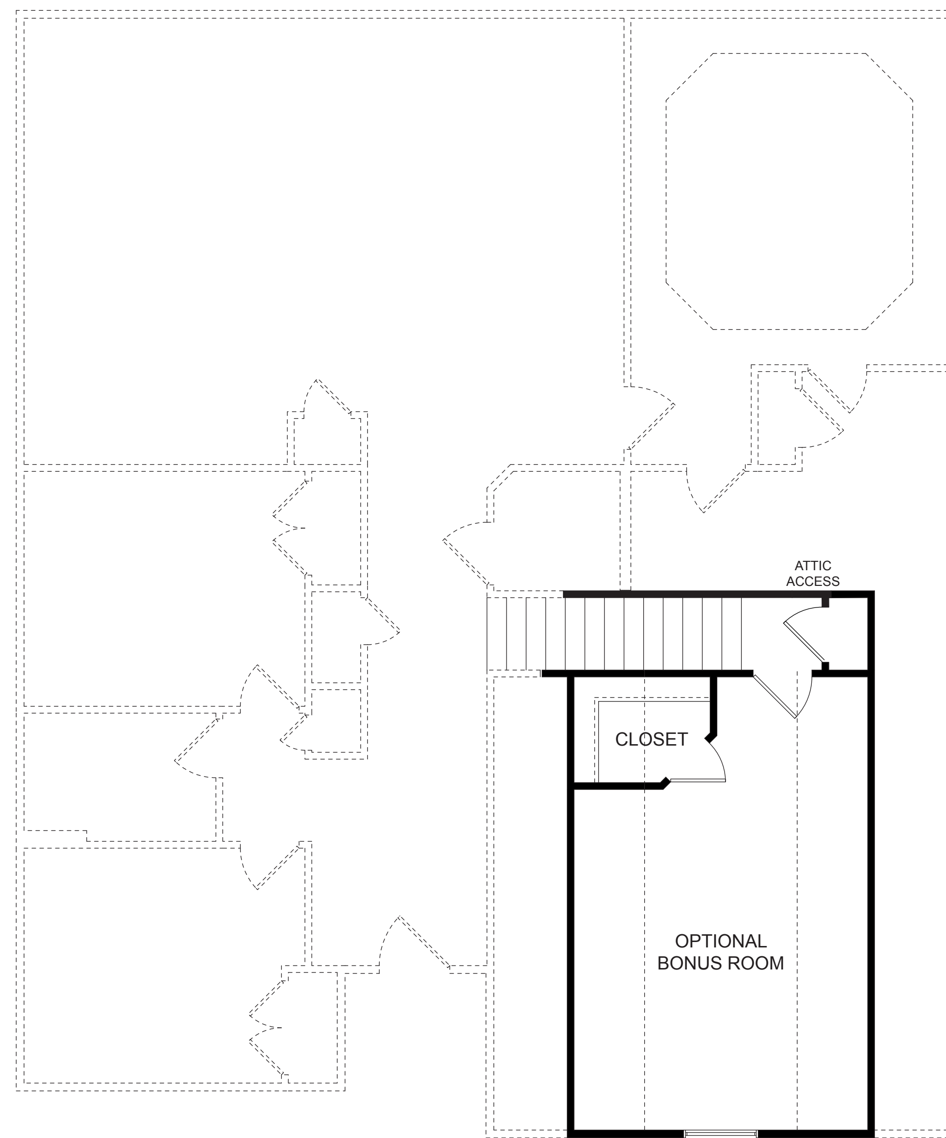
OPTIONAL SECOND FLOOR PLAN 227 SQ. FT.
